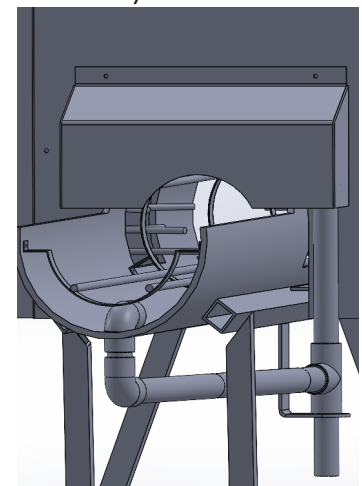
Water circuit
